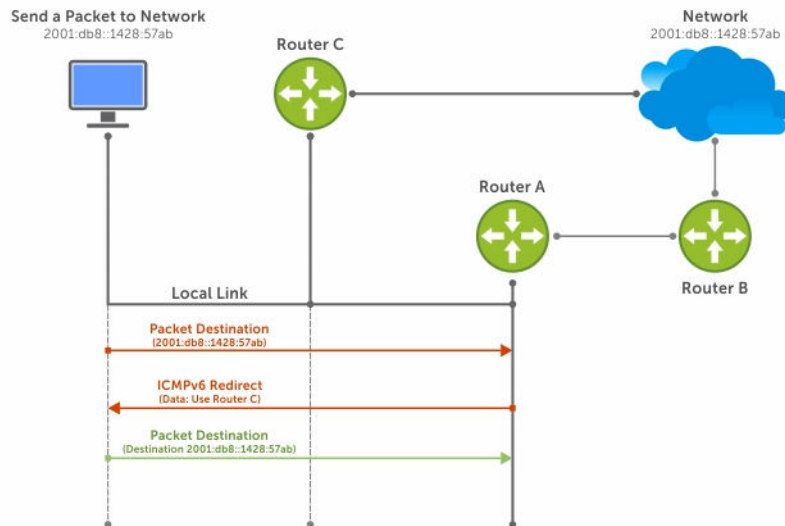
Figure 49. NDP Router Redirect
